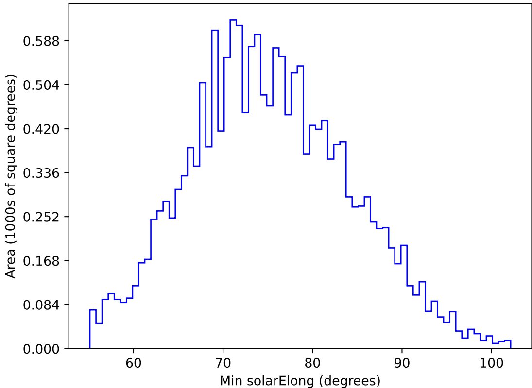
internal_u_expt30_nscale1.2v3.4_10yrs WFD g band: Min solarElong
