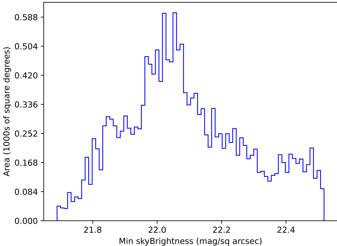
internal_u_expt30_nscale1.2v3.4_10yrs WFD u band: Min skyBrightness
