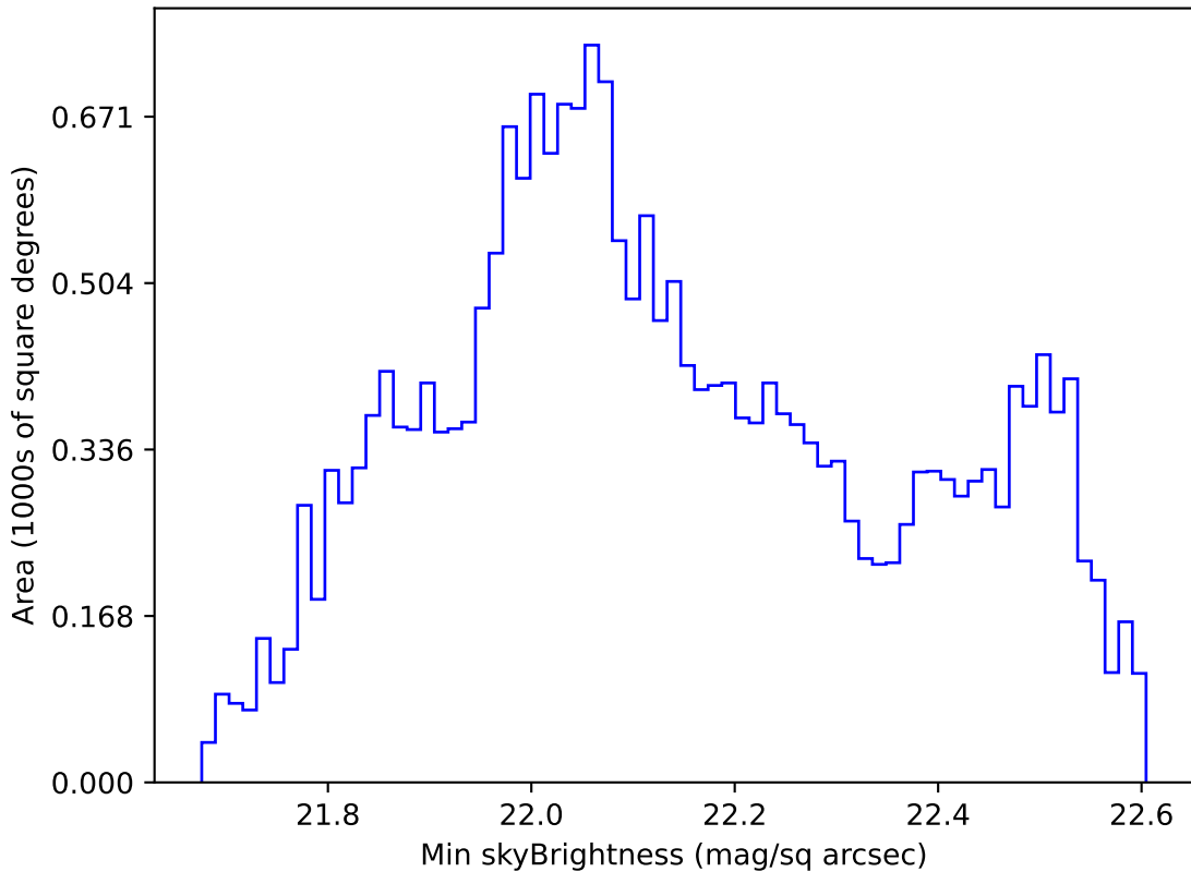
internal_u_expt30_nscale1.2v3.4_10yrs All sky u band: Min skyBrightness
