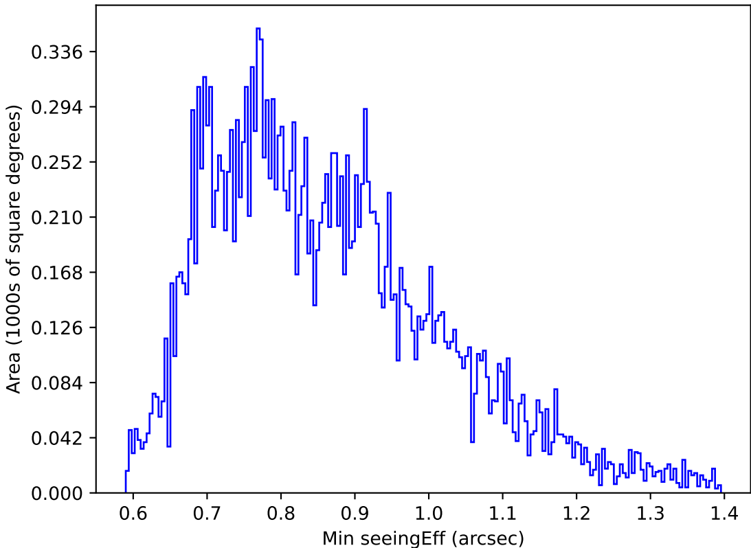
internal_u_expt30_nscale1.2v3.4_10yrs Yr 1 u band: Min seeingEff
