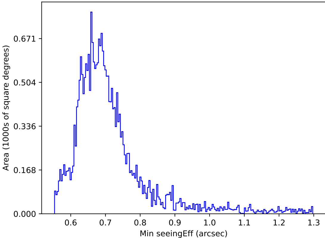
internal_u_expt30_nscale1.2v3.4_10yrs Yr 1 r band: Min seeingEff
