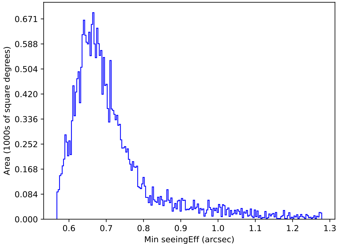
internal_u_expt30_nscale1.2v3.4_10yrs Yr 1 i band: Min seeingEff
