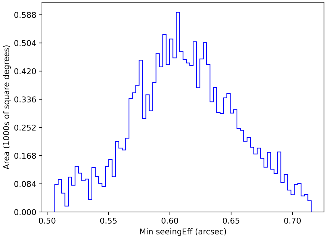
internal_u_expt30_nscale1.2v3.4_10yrs WFD z band: Min seeingEff
