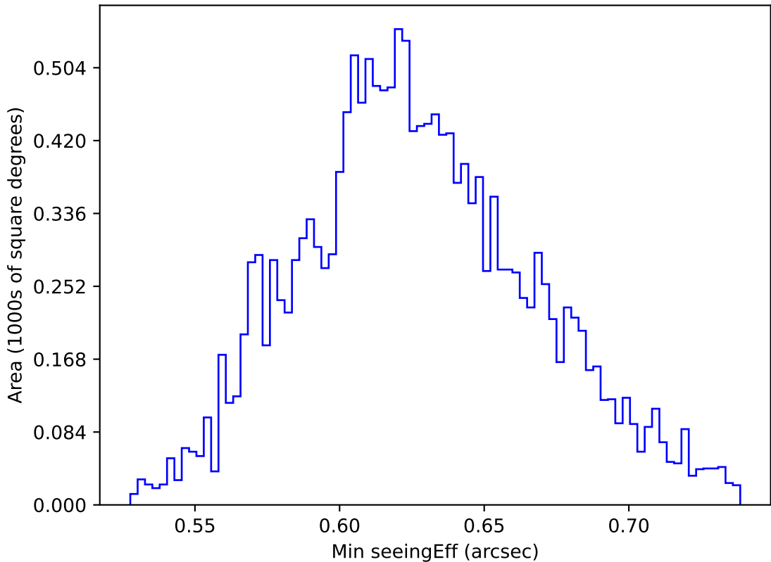
internal_u_expt30_nscale1.2v3.4_10yrs WFD y band: Min seeingEff
