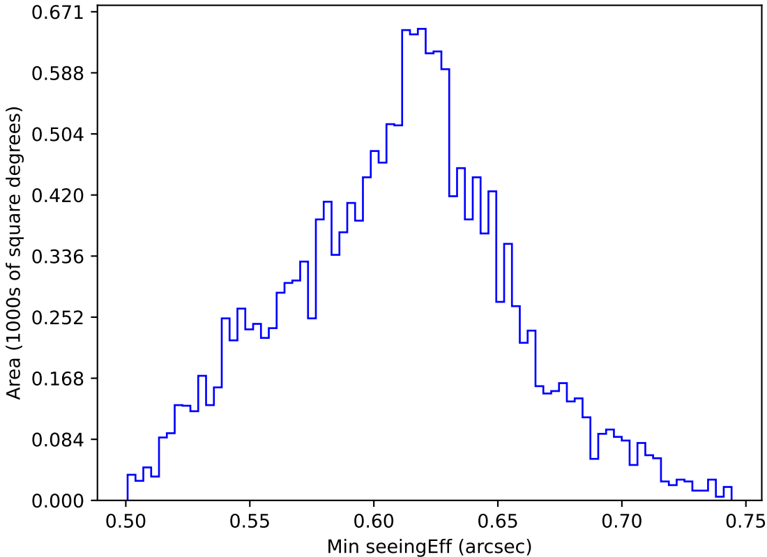
internal_u_expt30_nscale1.2v3.4_10yrs WFD r band: Min seeingEff
