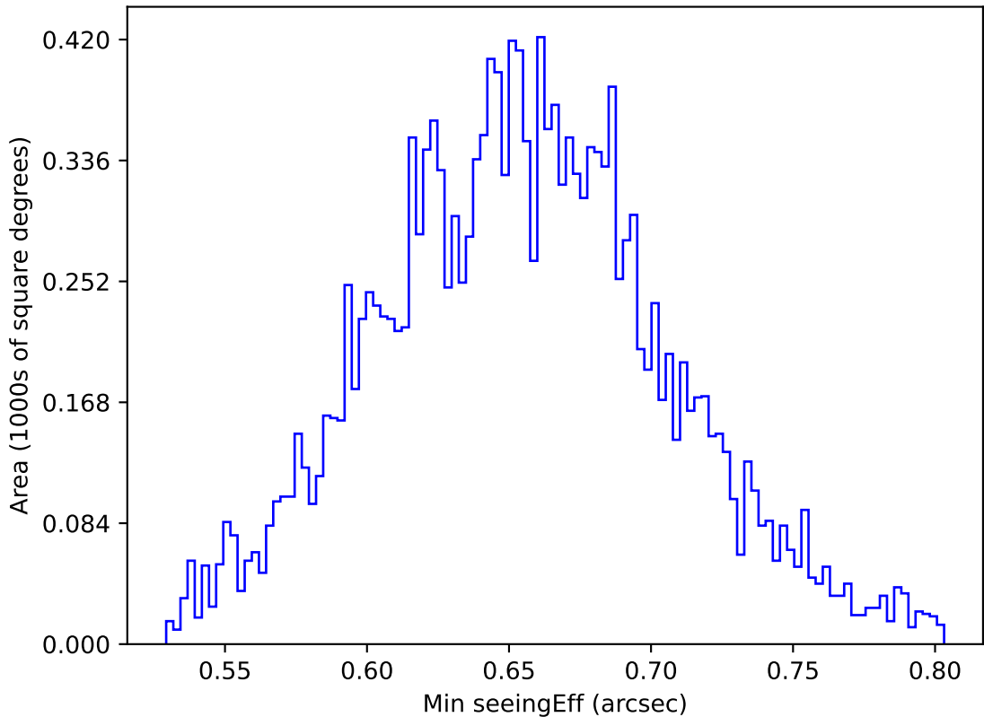
internal_u_expt30_nscale1.2v3.4_10yrs WFD g band: Min seeingEff
