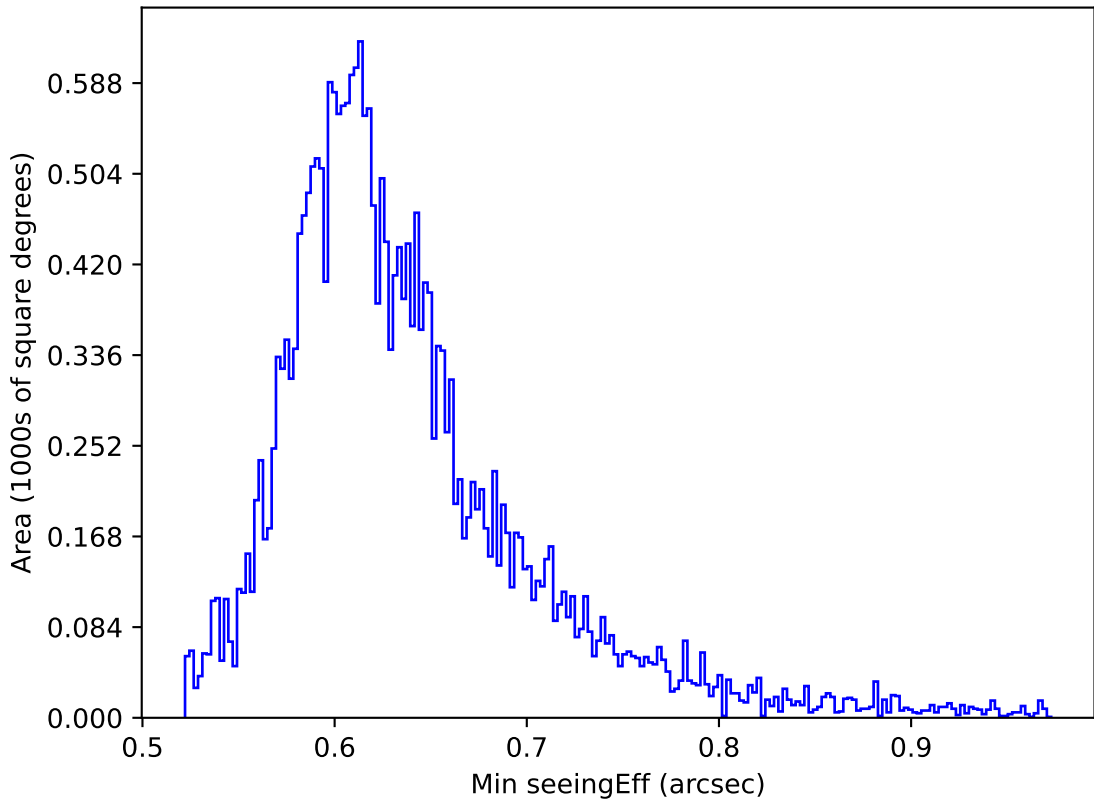
internal_u_expt30_nscale1.2v3.4_10yrs All sky i band: Min seeingEff
