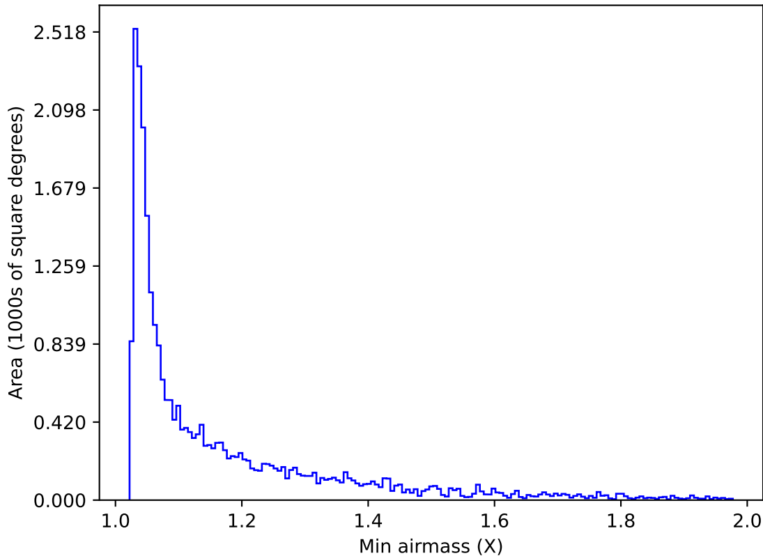
internal_u_expt30_nscale1.2v3.4_10yrs Yr 1 z band: Min airmass
