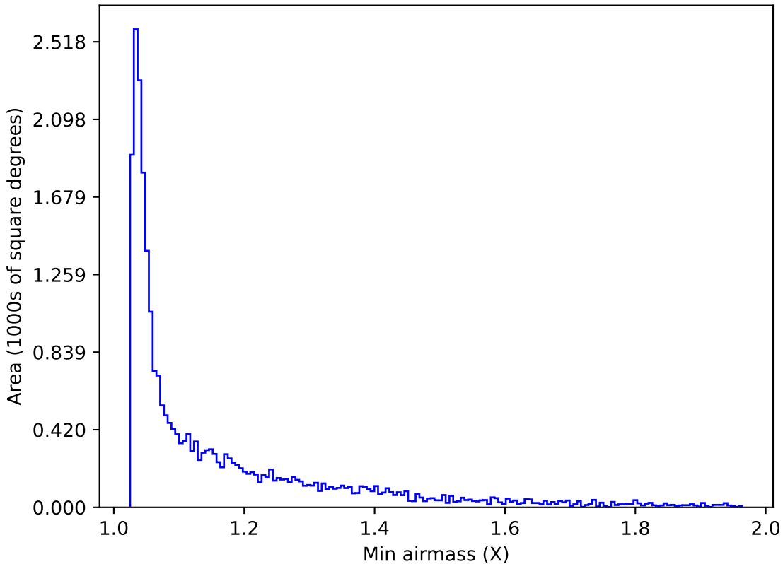
internal_u_expt30_nscale1.2v3.4_10yrs Yr 1 i band: Min airmass
