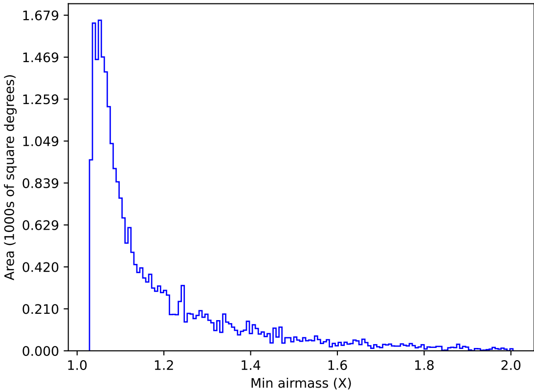
internal_u_expt30_nscale1.2v3.4_10yrs Yr 1 g band: Min airmass
