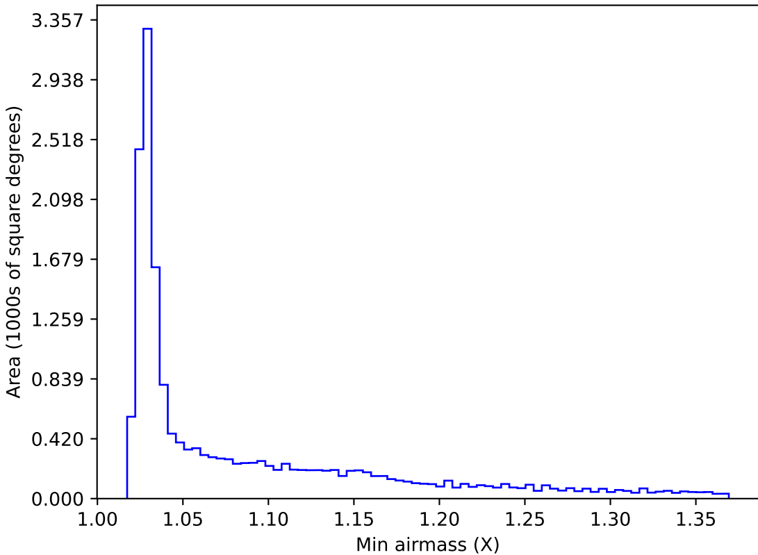
internal_u_expt30_nscale1.2v3.4_10yrs WFD z band: Min airmass
