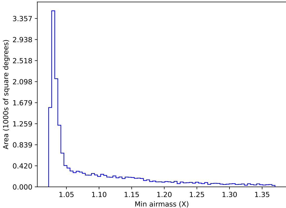
internal_u_expt30_nscale1.2v3.4_10yrs WFD y band: Min airmass
