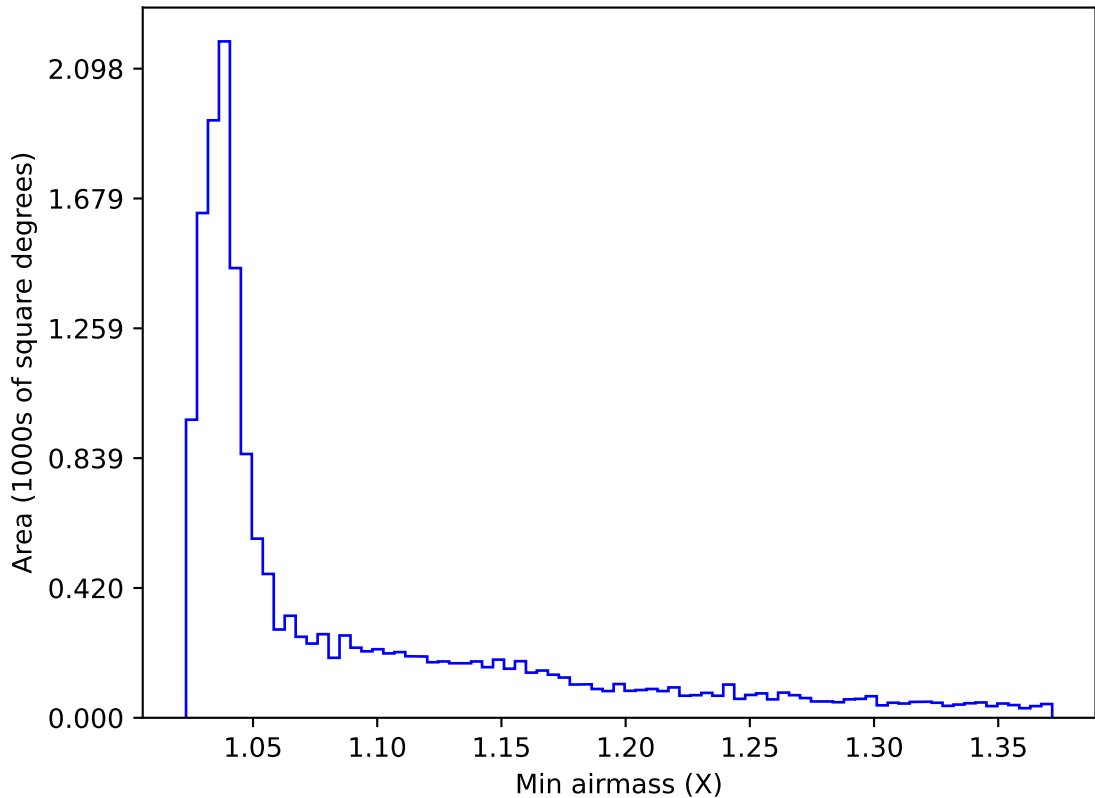
internal_u_expt30_nscale1.2v3.4_10yrs WFD g band: Min airmass
