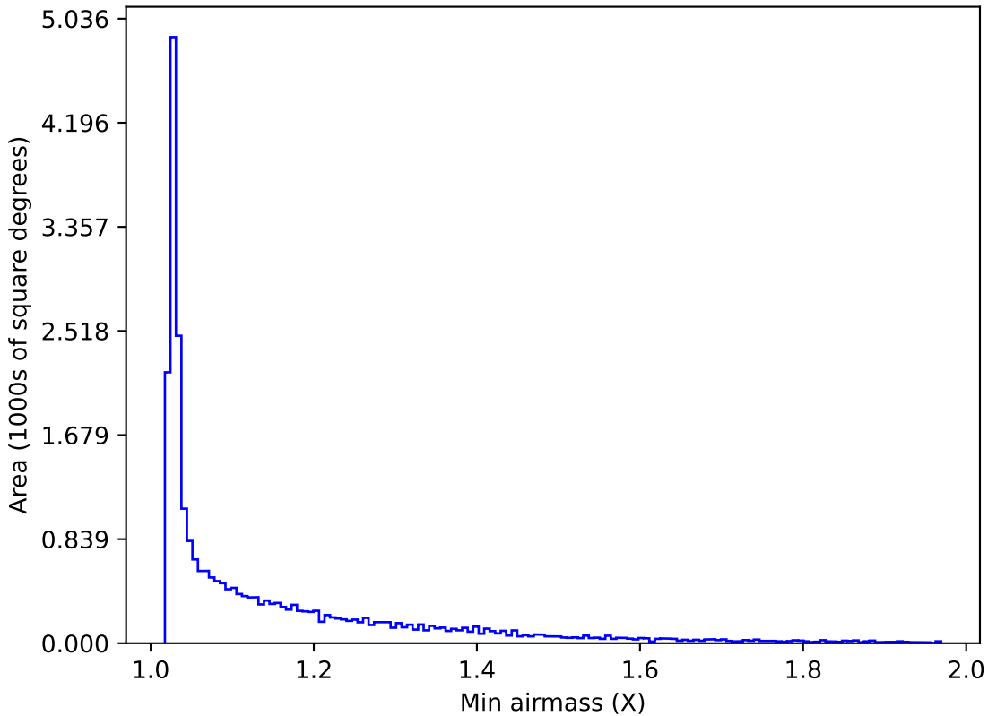
internal_u_expt30_nscale1.2v3.4_10yrs All sky r band: Min airmass
