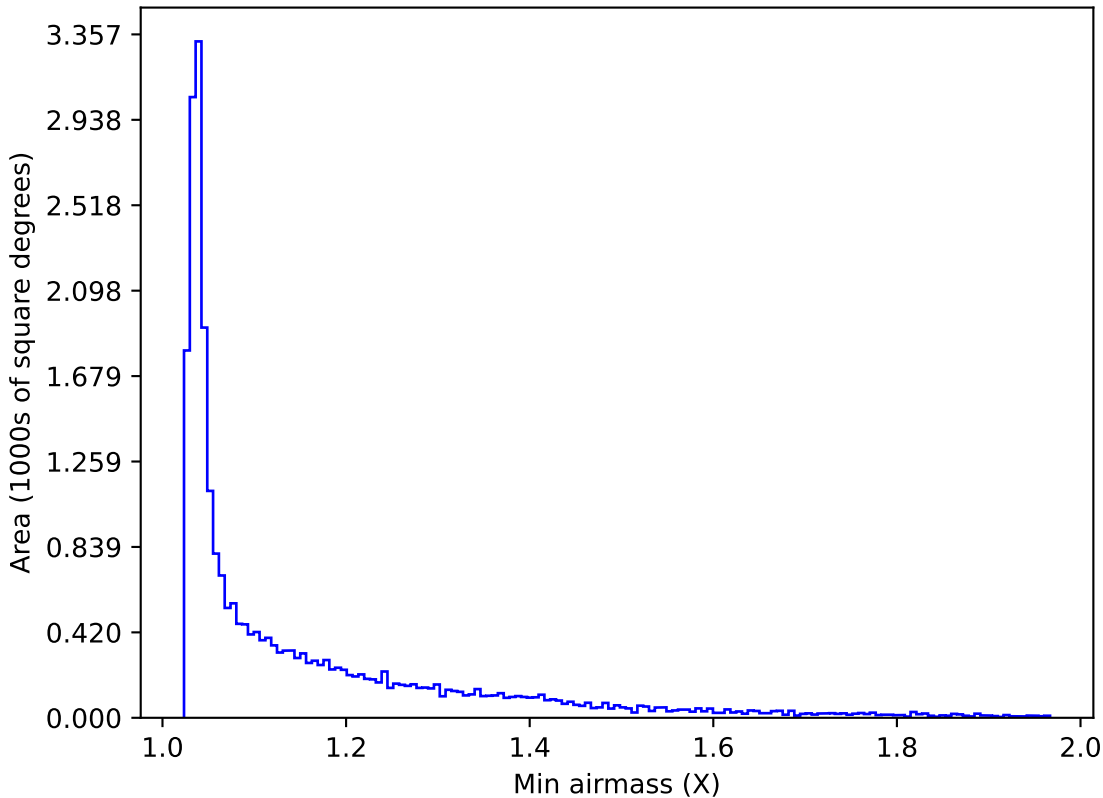
internal_u_expt30_nscale1.2v3.4_10yrs All sky g band: Min airmass
