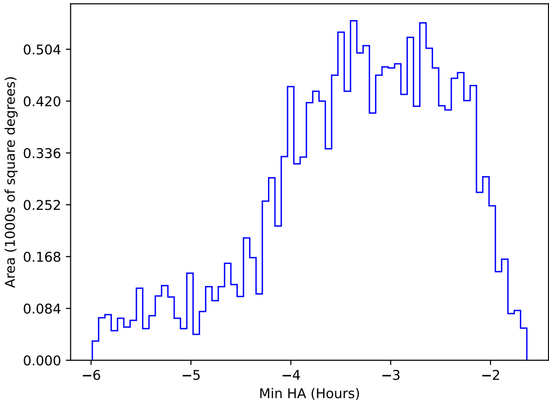
internal_u_expt30_nscale1.2v3.4_10yrs WFD u band: Min HA
