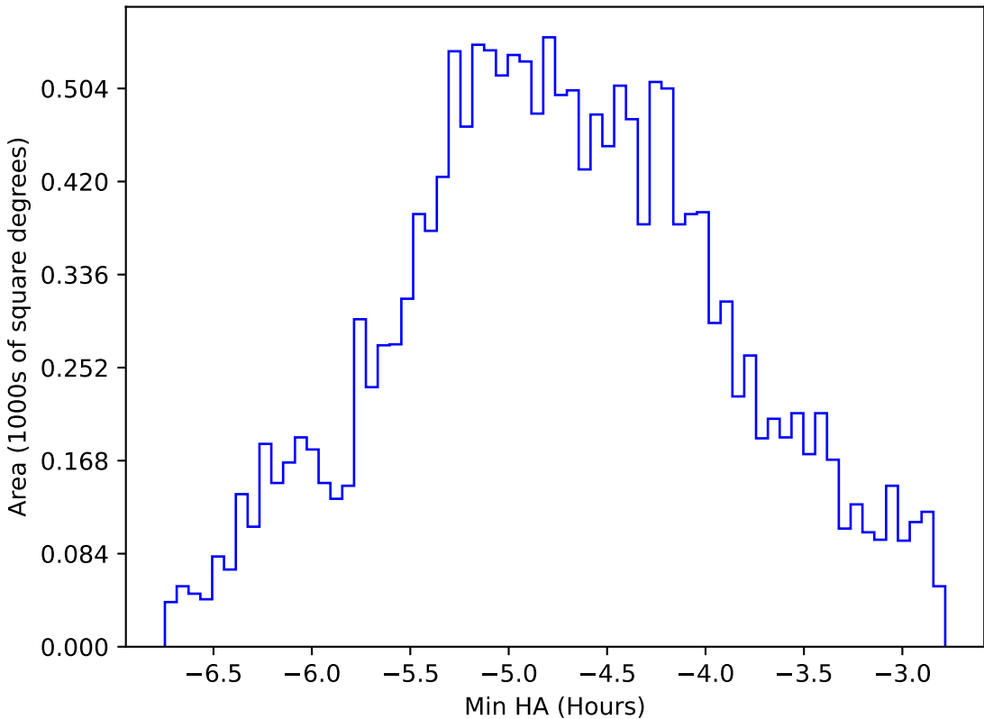
internal_u_expt30_nscale1.2v3.4_10yrs WFD all bands: Min HA
