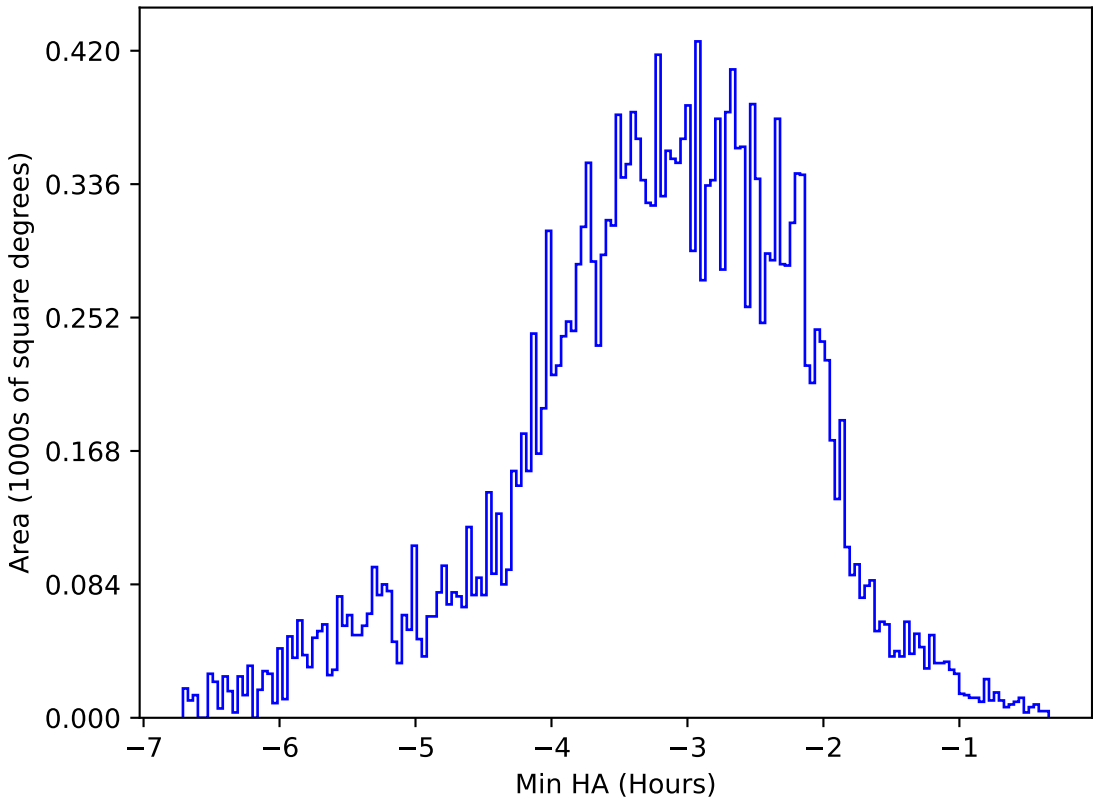
internal_u_expt30_nscale1.2v3.4_10yrs All sky u band: Min HA
