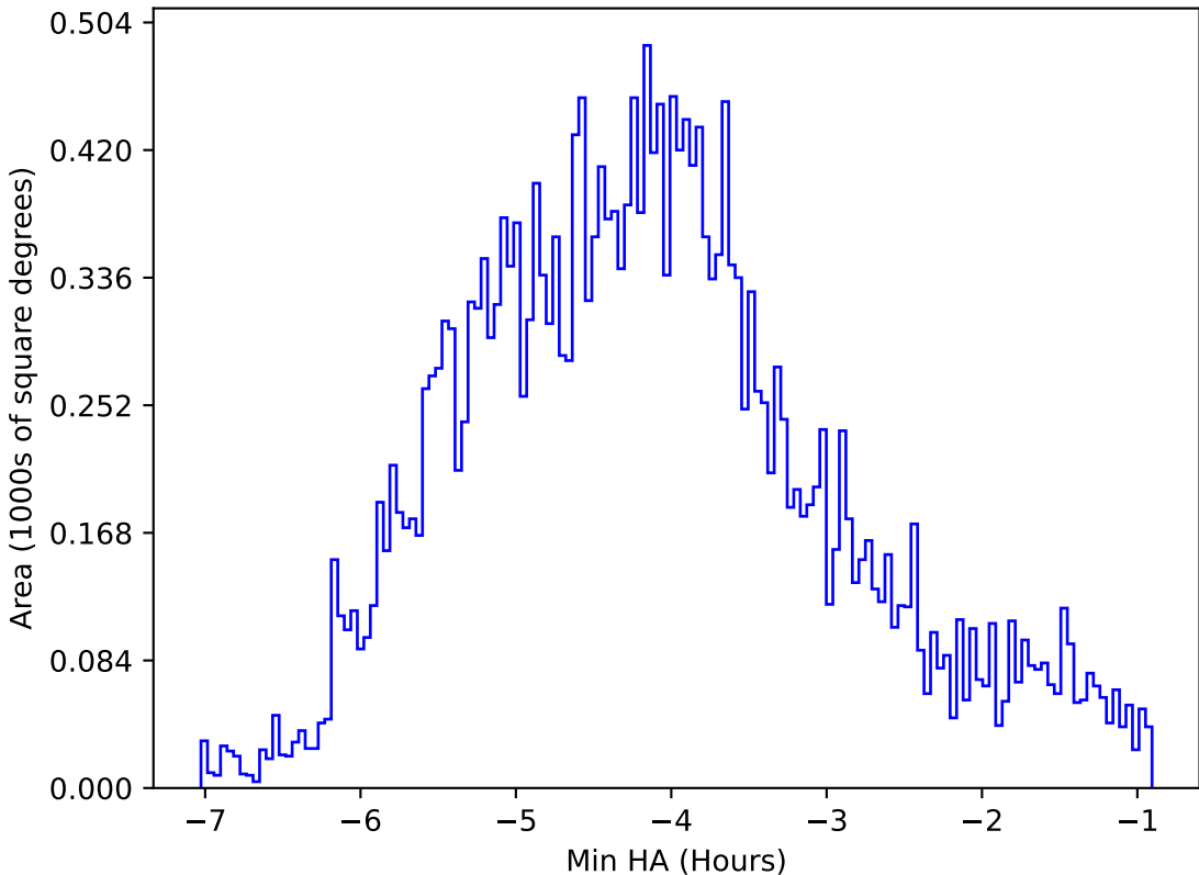
internal_u_expt30_nscale1.2v3.4_10yrs All sky r band: Min HA
