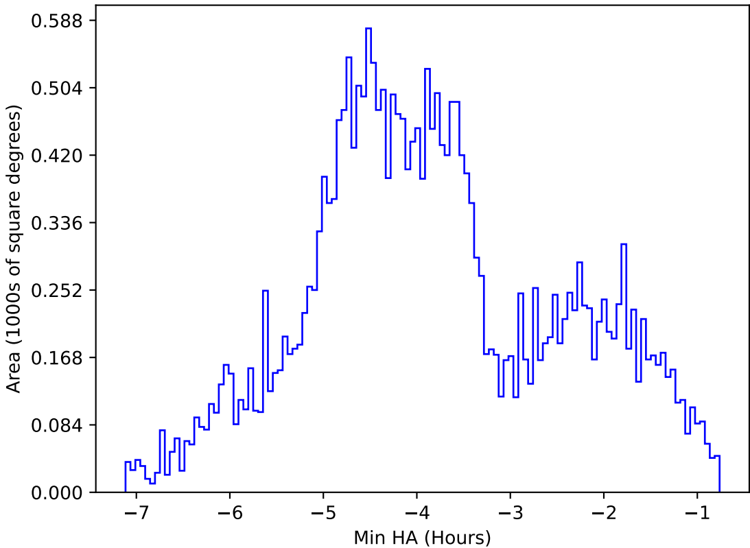
internal_u_expt30_nscale1.2v3.4_10yrs All sky g band: Min HA
