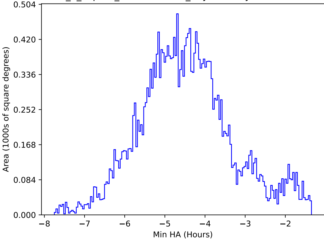
internal_u_expt30_nscale1.2v3.4_10yrs All sky all bands: Min HA
