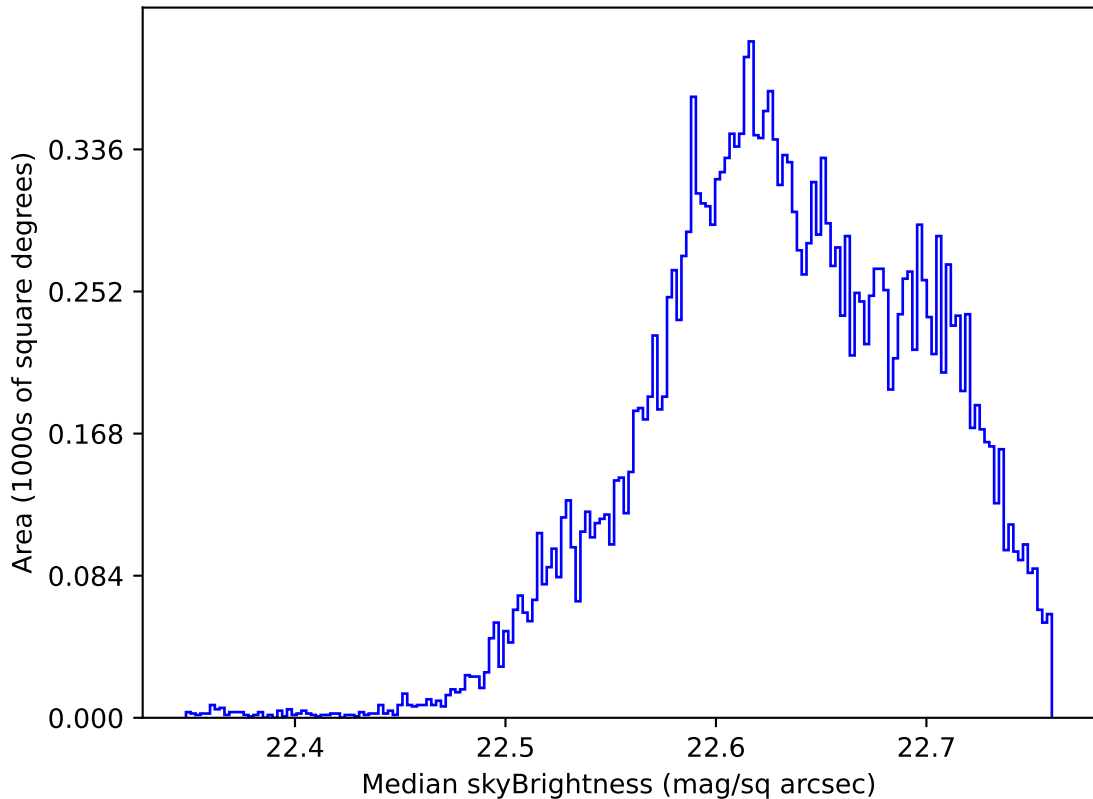
internal_u_expt30_nscale1.2v3.4_10yrs Yr 1 u band: Median skyBrightness
