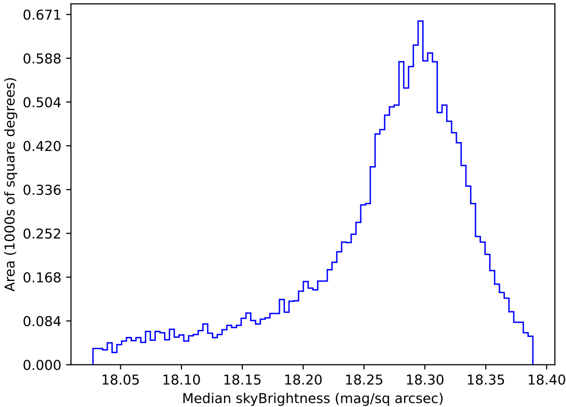
internal_u_expt30_nscale1.2v3.4_10yrs WFD y band: Median skyBrightness
