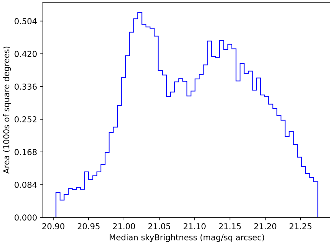
internal_u_expt30_nscale1.2v3.4_10yrs WFD r band: Median skyBrightness
