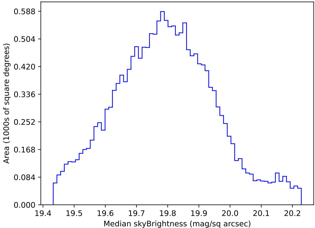
internal_u_expt30_nscale1.2v3.4_10yrs WFD all bands: Median skyBrightness
