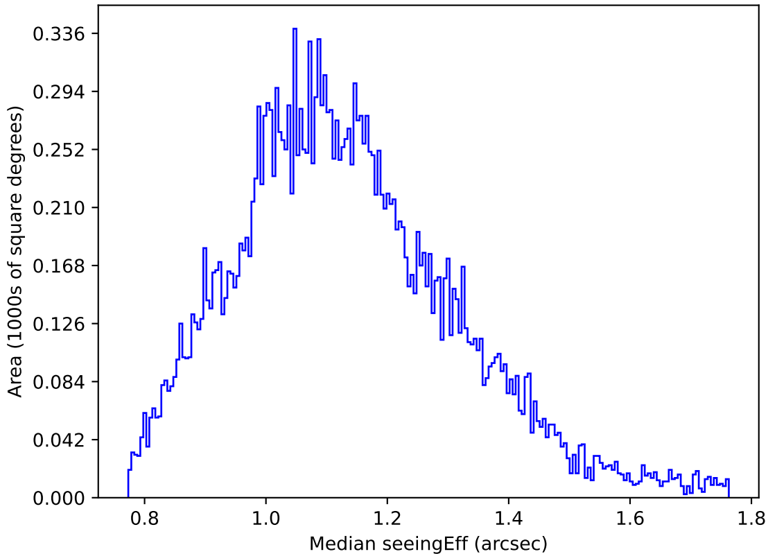
internal_u_expt30_nscale1.2v3.4_10yrs Yr 1 u band: Median seeingEff
