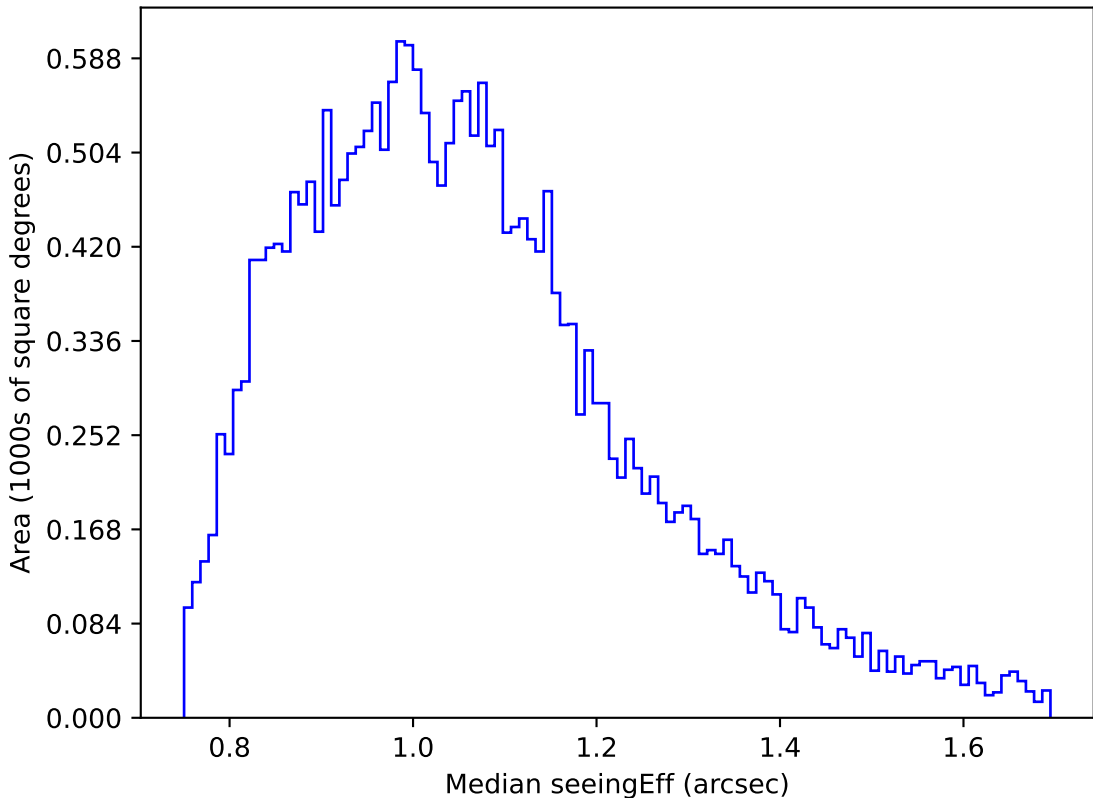
internal_u_expt30_nscale1.2v3.4_10yrs Yr 1 g band: Median seeingEff
