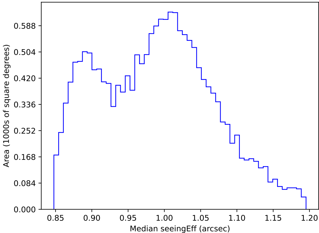
internal_u_expt30_nscale1.2v3.4_10yrs WFD i band: Median seeingEff
