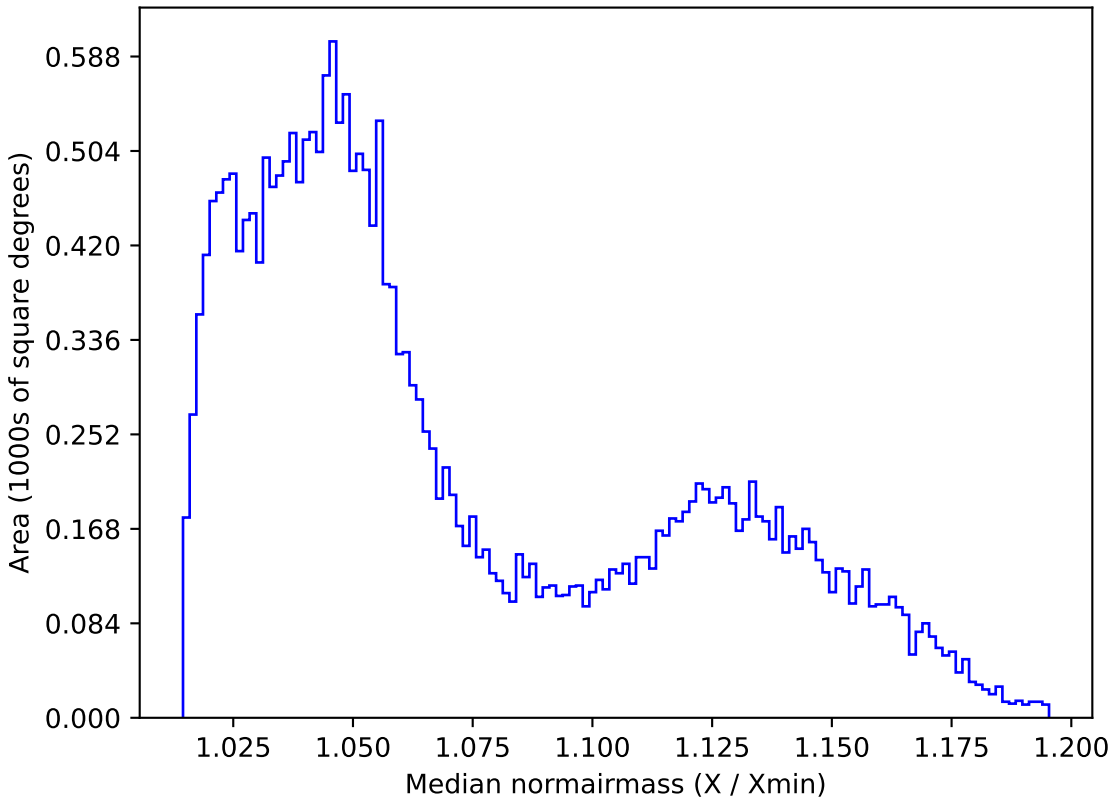
internal_u_expt30_nscale1.2v3.4_10yrs All sky r band: Median normairmass
