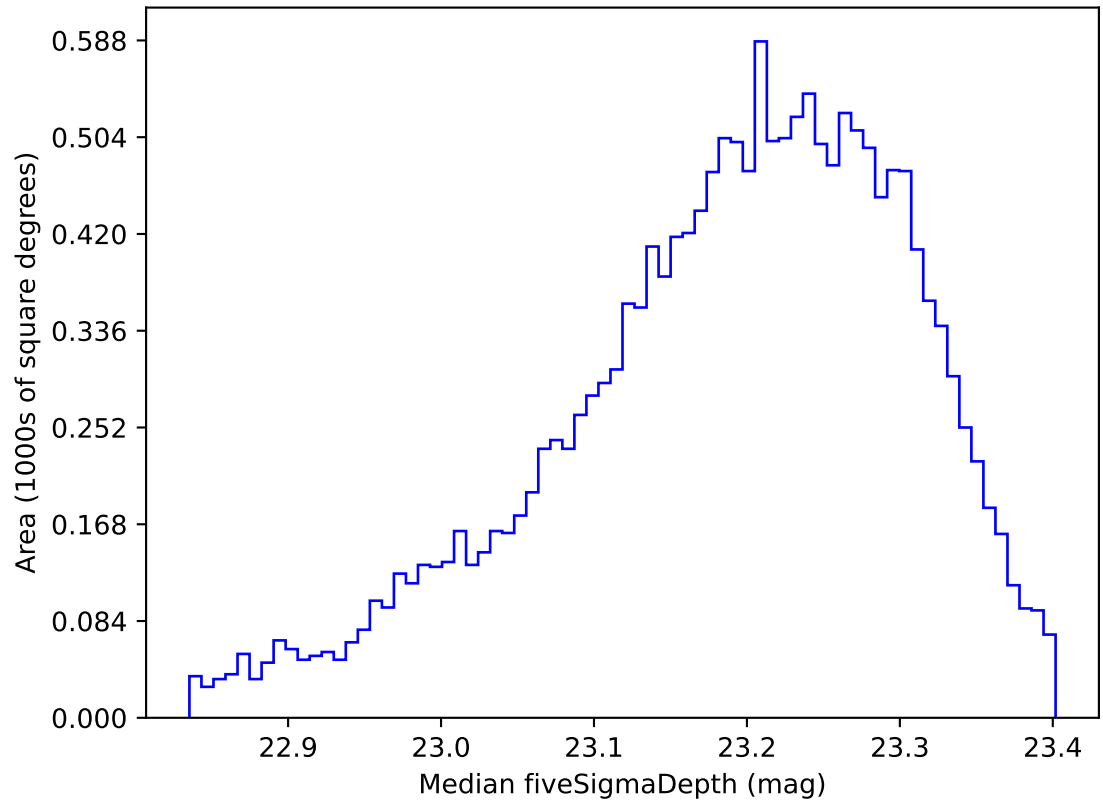
internal_u_expt30_nscale1.2v3.4_10yrs WFD u band: Median fiveSigmaDepth
