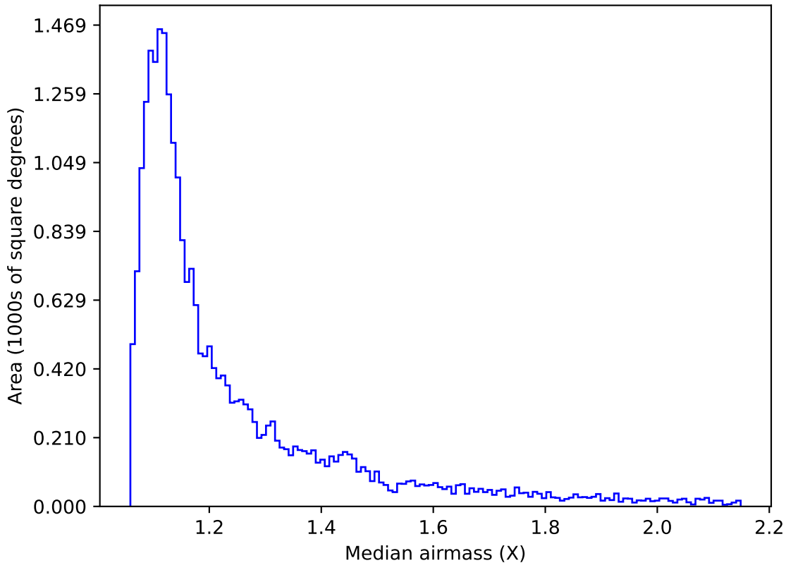
internal_u_expt30_nscale1.2v3.4_10yrs Yr 1 r band: Median airmass
