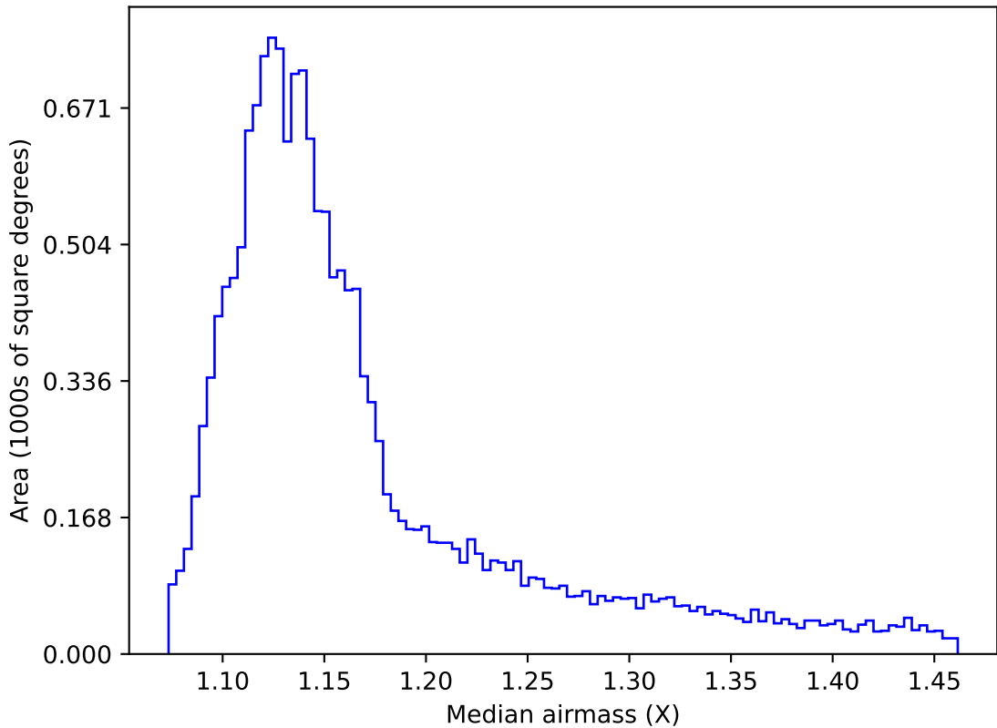
internal_u_expt30_nscale1.2v3.4_10yrs WFD r band: Median airmass
