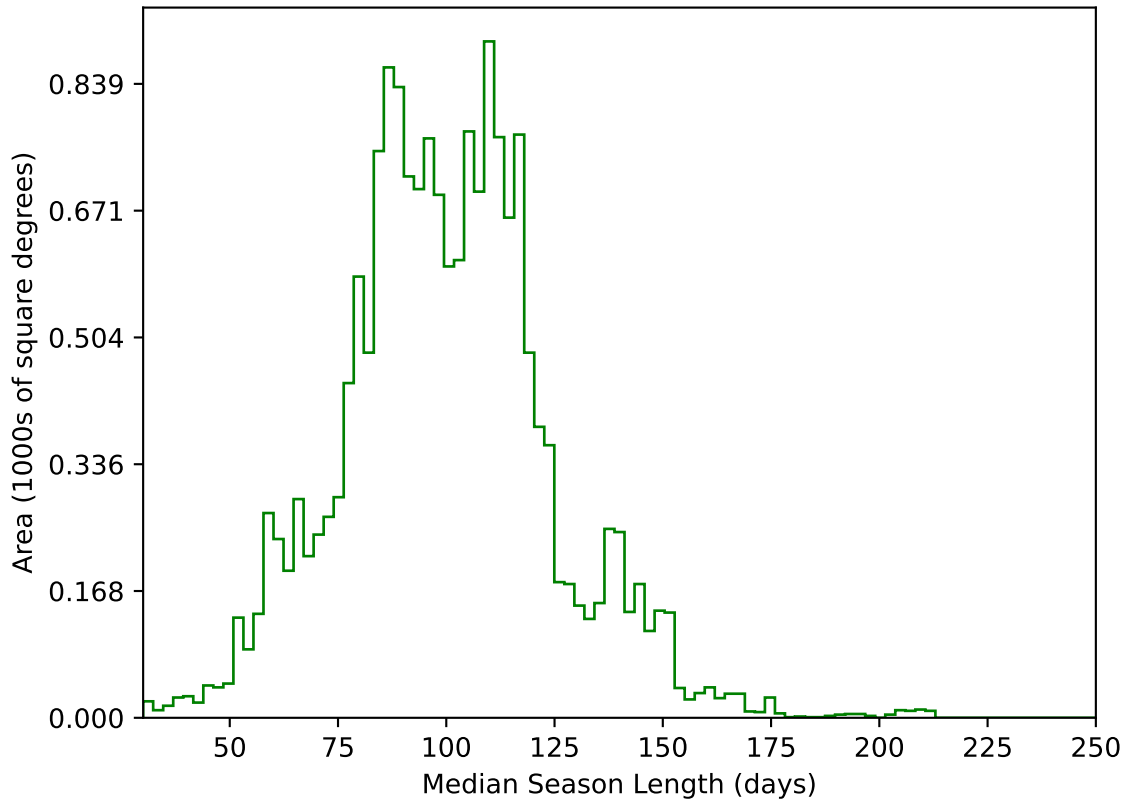
internal_u_expt30_nscale1.2v3.4_10yrs WFD g band: Median Season Length
