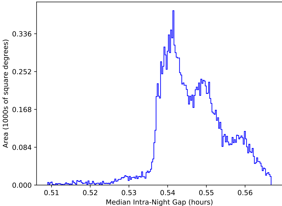
internal_u_expt30_nscale1.2v3.4_10yrs WFD: Median Intra-Night Gap
