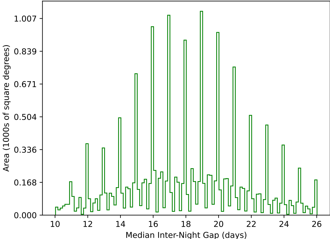
internal_u_expt30_nscale1.2v3.4_10yrs WFD g band: Median Inter-Night Gap
