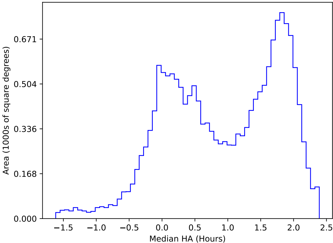
internal_u_expt30_nscale1.2v3.4_10yrs WFD u band: Median HA
