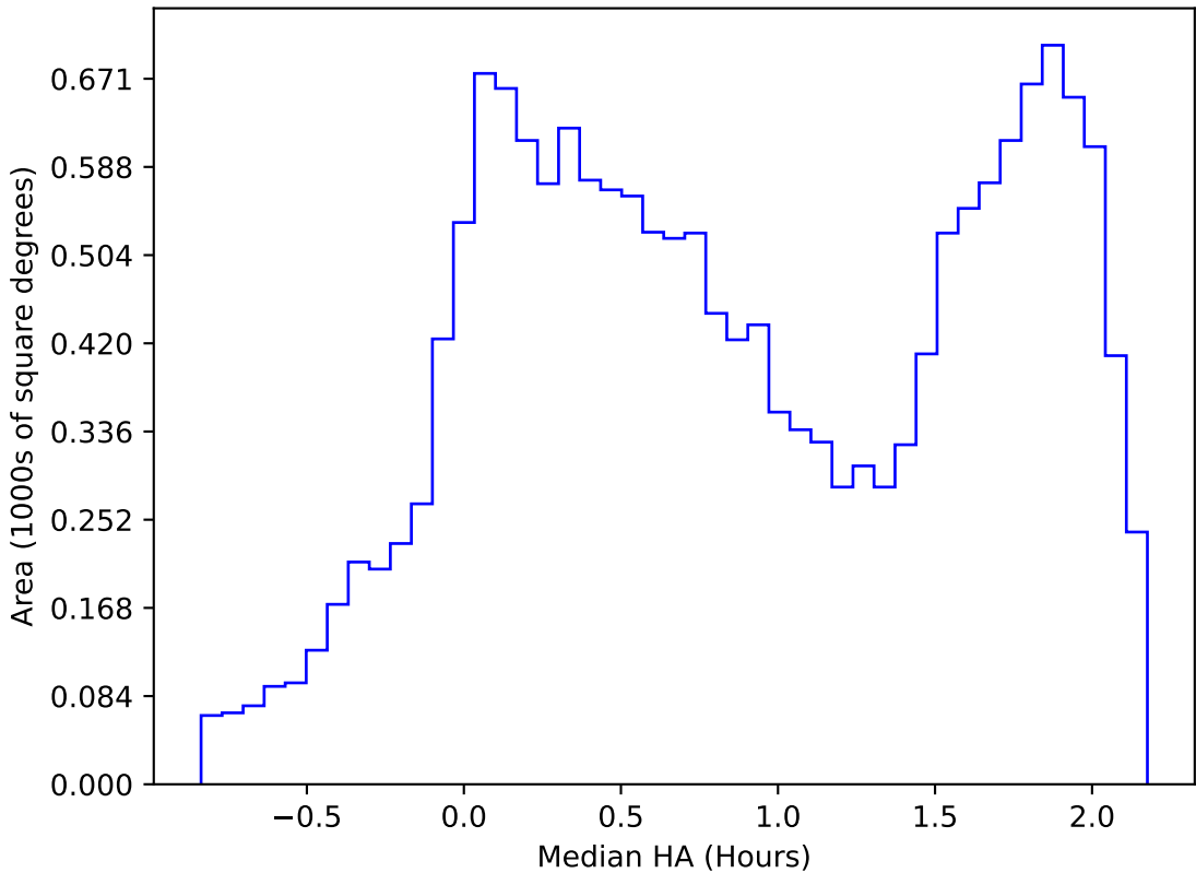
internal_u_expt30_nscale1.2v3.4_10yrs WFD r band: Median HA
