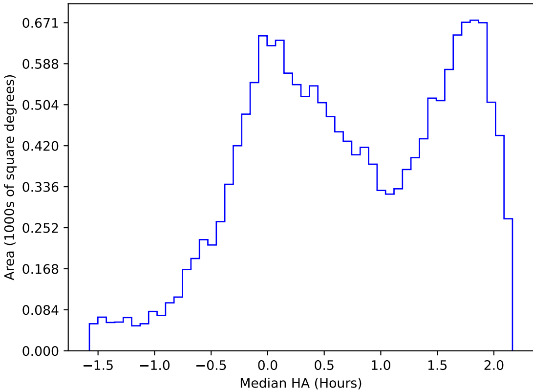
internal_u_expt30_nscale1.2v3.4_10yrs WFD g band: Median HA
