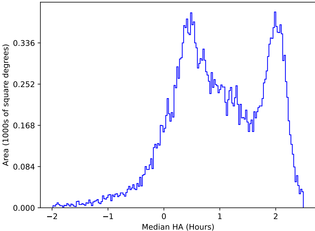
internal_u_expt30_nscale1.2v3.4_10yrs All sky z band: Median HA
