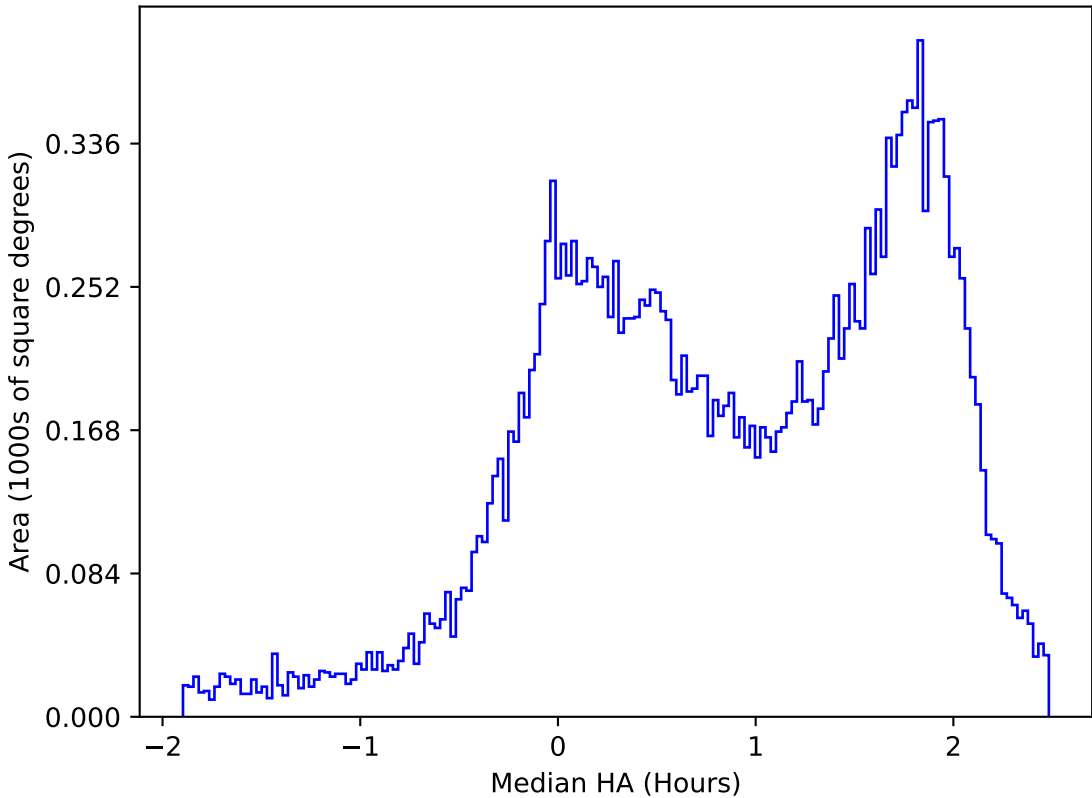
internal_u_expt30_nscale1.2v3.4_10yrs All sky u band: Median HA
