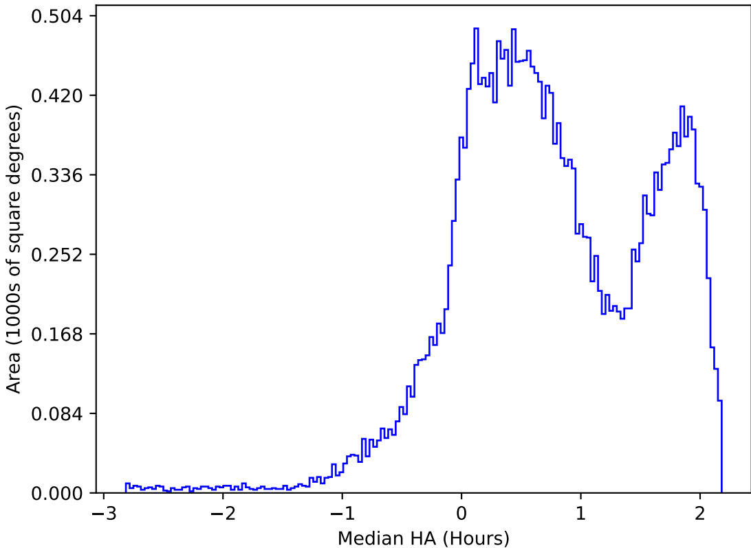
internal_u_expt30_nscale1.2v3.4_10yrs All sky r band: Median HA
