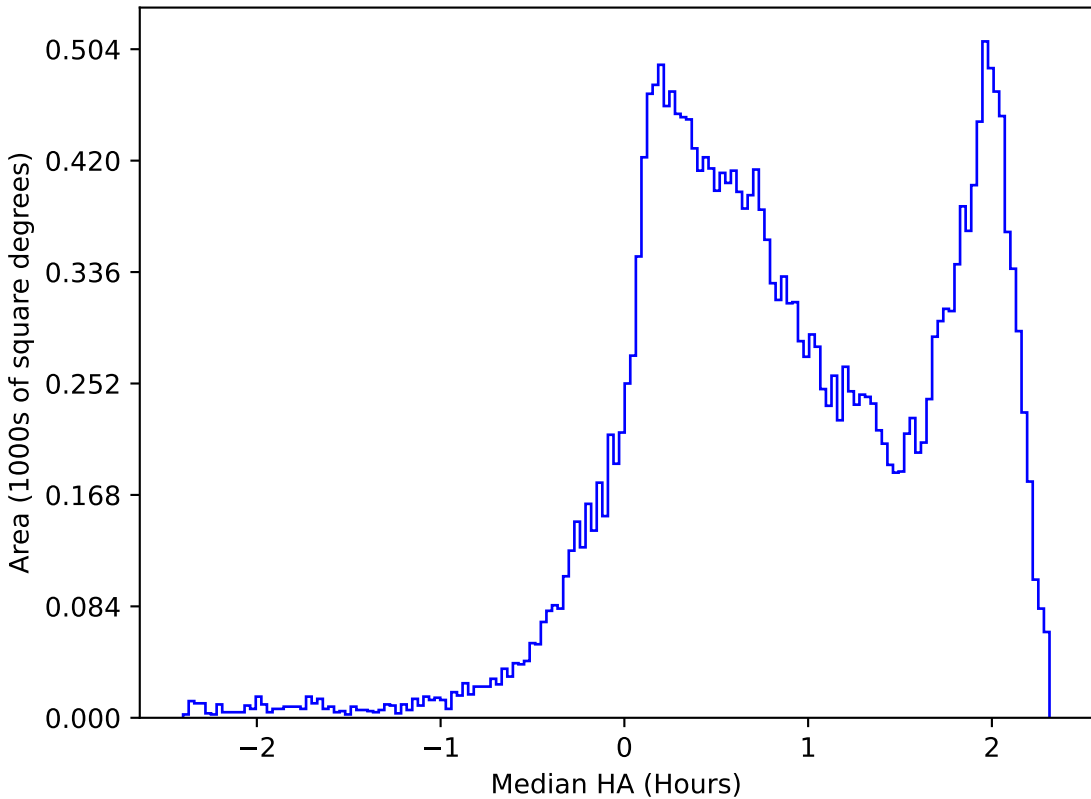
internal_u_expt30_nscale1.2v3.4_10yrs All sky i band: Median HA
