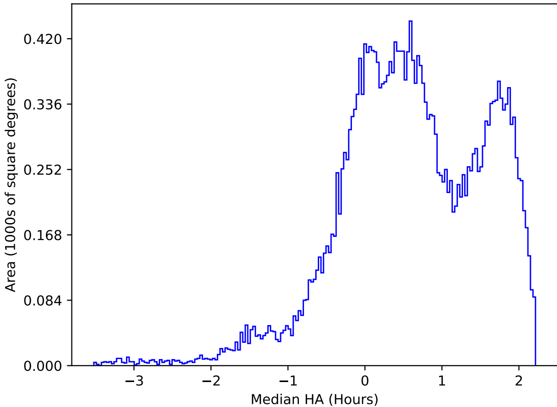
internal_u_expt30_nscale1.2v3.4_10yrs All sky g band: Median HA
