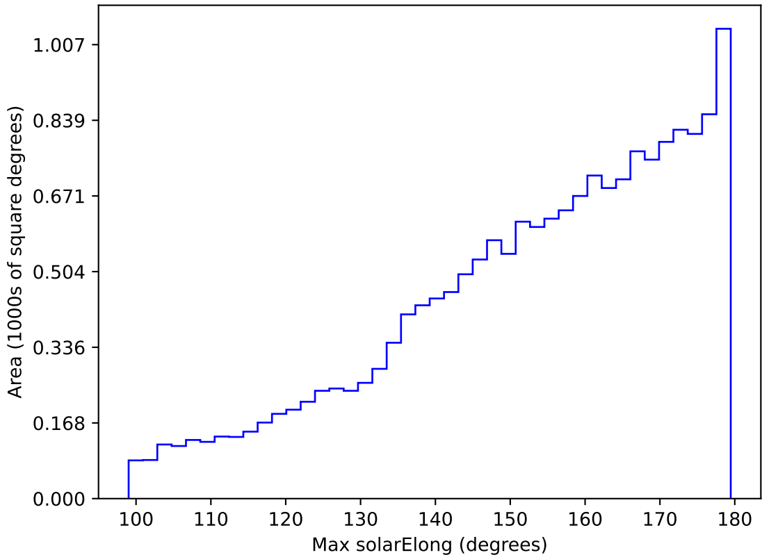
internal_u_expt30_nscale1.2v3.4_10yrs WFD r band: Max solarElong
