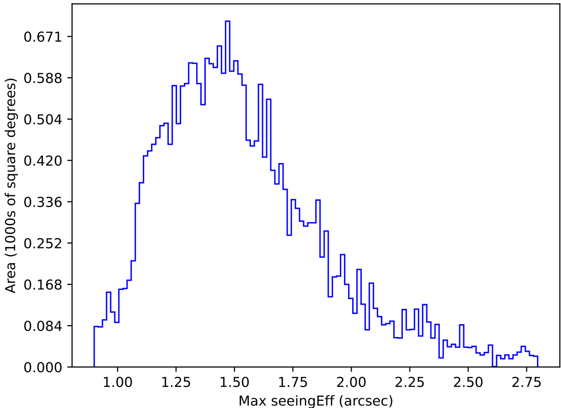
internal_u_expt30_nscale1.2v3.4_10yrs Yr 1 z band: Max seeingEff
