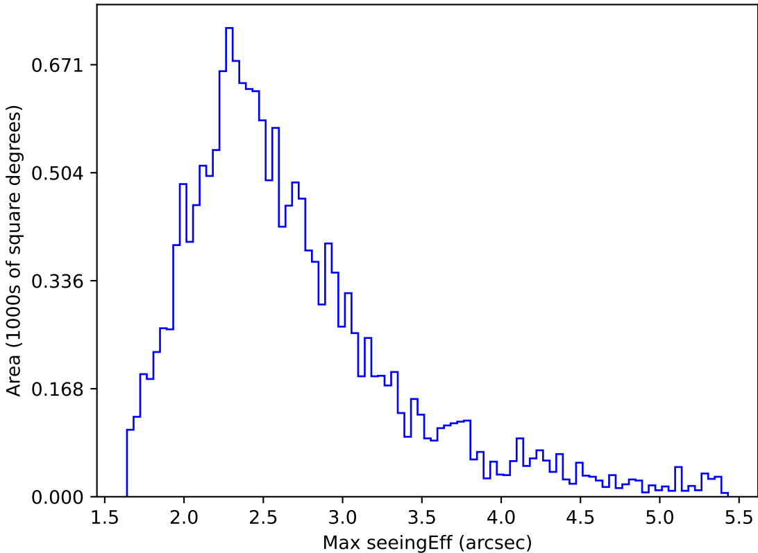
internal_u_expt30_nscale1.2v3.4_10yrs WFD z band: Max seeingEff
